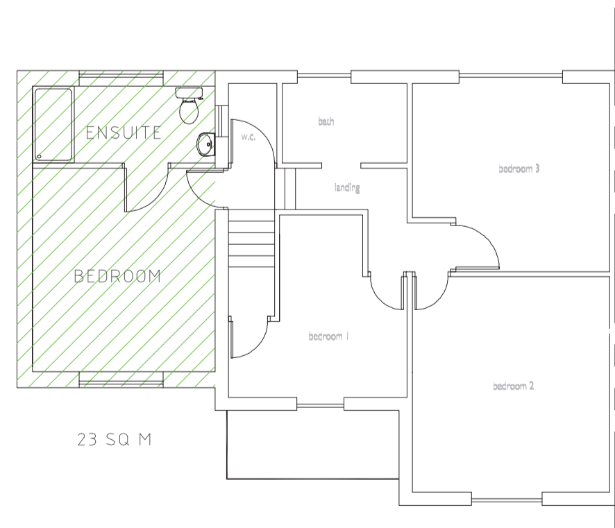
PROPOSED 1ST FLOOR PLAN
